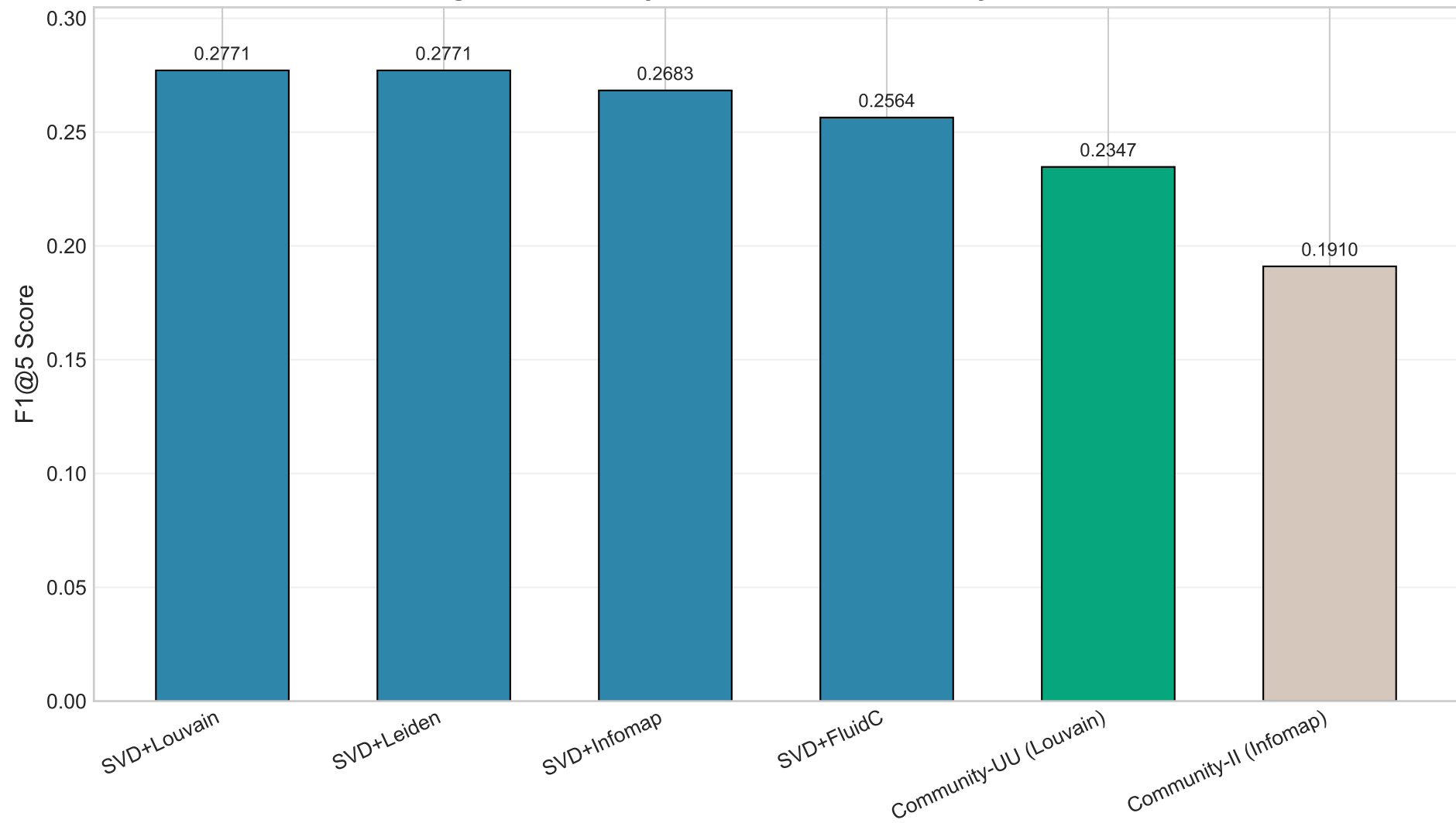
Figure 34: SVD Hybrids vs. Pure Community Baselines
